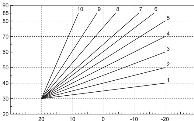
fig. 32- Compensation curves
