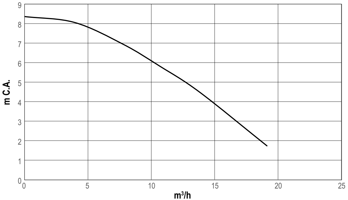
fig. 121 - Head diagram
