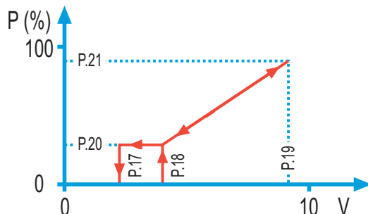
fig. 53- Control in power
