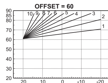
fig. 33- Compensation curve parallel offset
